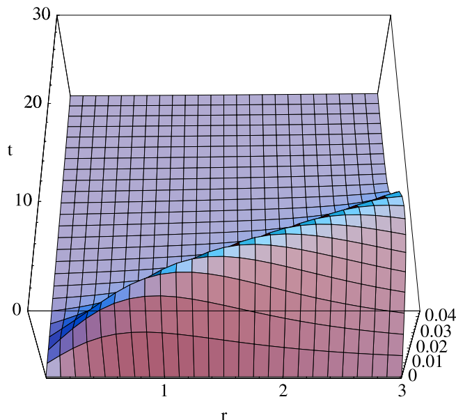
Figure 4: A result of numerical simulation in spherical symmetry ( s = 2 ) with an external gravitational potential. The variable A_r is plotted as a function of r and t . Again, we observe the absence of late time caustics.
