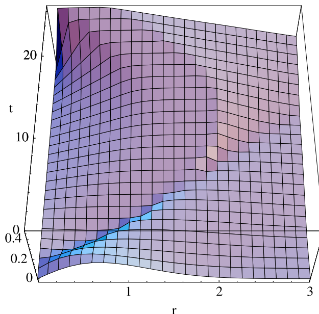
Figure 1: A result of numerical simulation for planar symmetry ( s = 0 ). The variable A_r is plotted as a function of r and t . After an initial bounce, a caustic singularity forms at late times. Note that in a realistic situation, we do not expect a system to exhibit planar symmetry.
