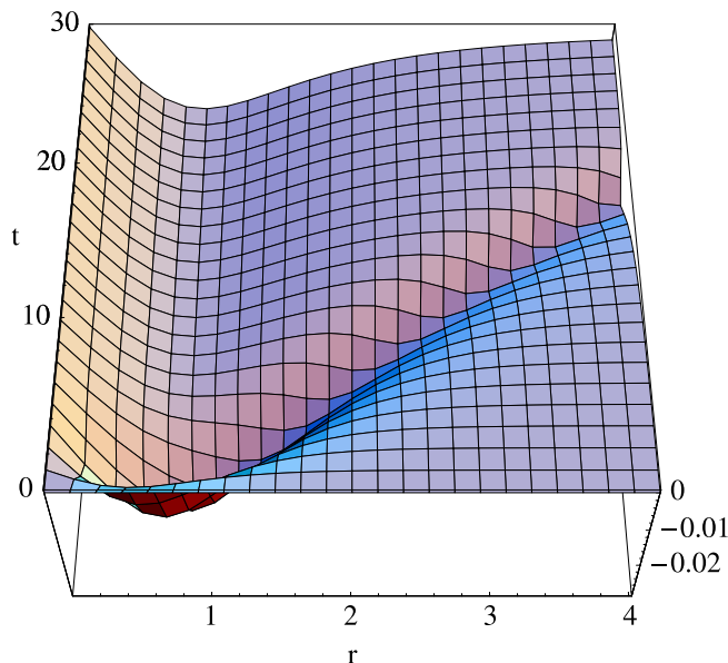
Figure 5: A result of numerical simulation in spherical symmetry ( s = 2 ) with an external gravitational potential. The variable E_r is plotted as a function of r and t . At late times, the “electric field” cancels the gravitational force, halting the accretion of the gauged ghost condensate and protecting the system from caustics.
