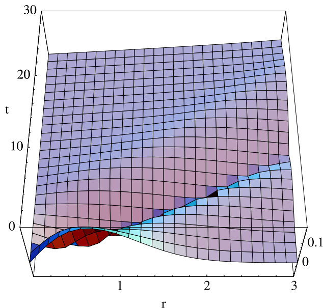
Figure 2: A result of numerical simulation in cylindrical symmetry ( s = 1 ). The variable A_r is plotted as a function of r and t . After an initial bounce, no caustics form at late times.
