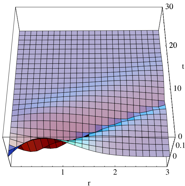
Figure 3: A result of numerical simulation in spherical symmetry ( s = 2 ). The variable A_r is plotted as a function of r and t . Like the case of cylindrical symmetry, there are no late time caustics.
